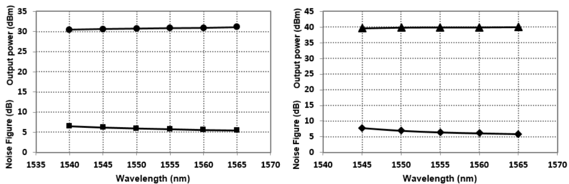
Fig. 3. Preliminary modelling results using conventional silica Er/Yb co-doped fibre for the two amplifier models foreseen within the project.
