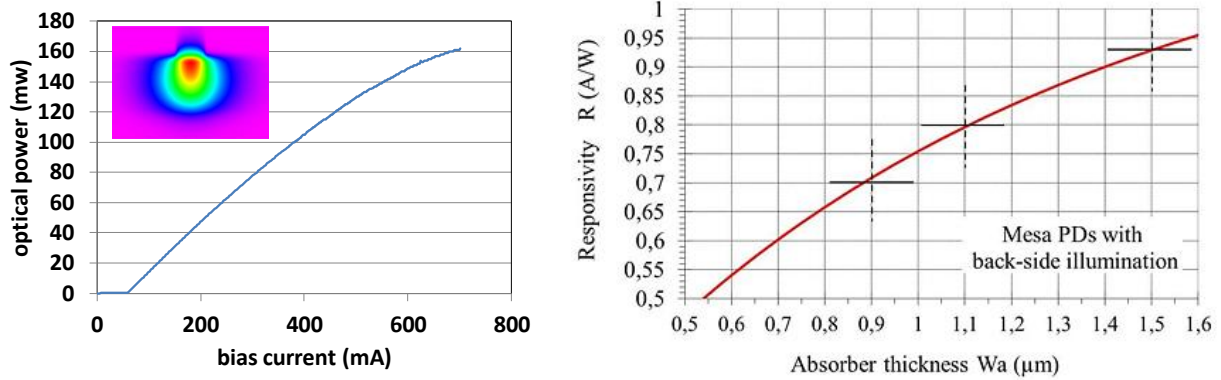
Fig. 2. (left) DFB experimental results from various devices within the 1 st fabrication run and (right) simulation of the back-side illuminated UTC photodiode versus absorber thickness ( W_a )
